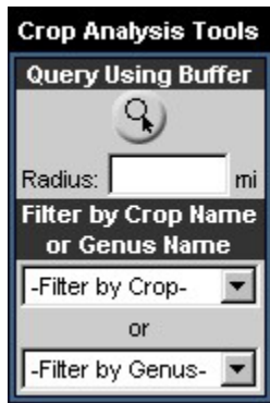
Buffer/Query Tool
